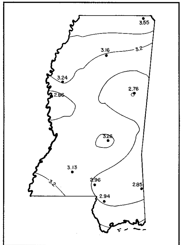
Figure 10. Average monthly precipitation pattern in Mississippi, October.
