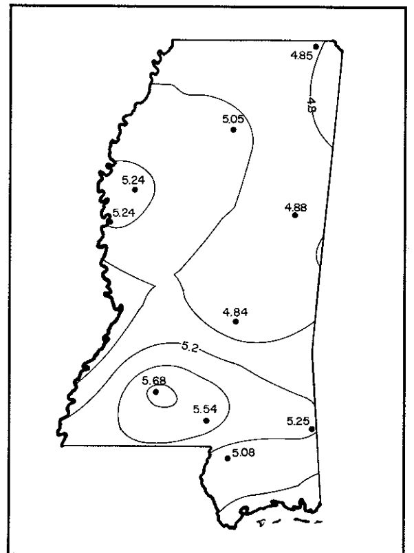
Figure 4. Average monthly precipitation pattern in Mississippi, April.
