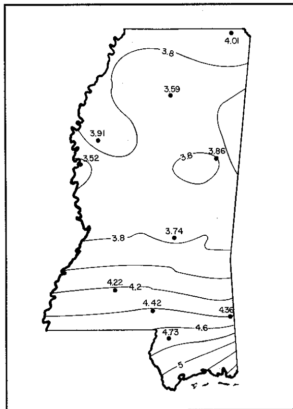
Figure 6. Average monthly precipitation pattern in Mississippi, June.
