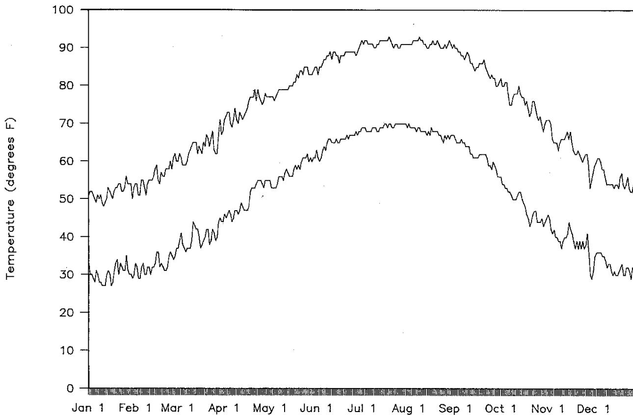
Figure 14. Average daily high and low temperatures, North Mississippi (Water Valley).
