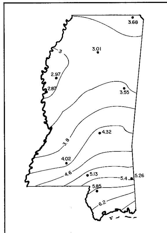
Figure 8. Average monthly precipitation pattern in Mississippi, August.
