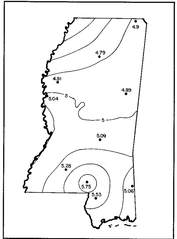
Figure 2. Average monthly precipitation pattern in Mississippi, February.
