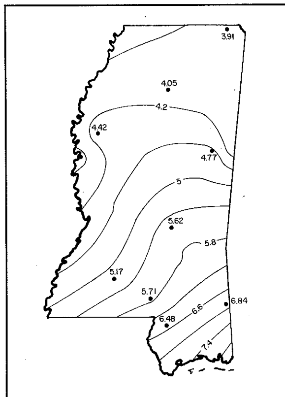
Figure 7. Average monthly precipitation pattern in Mississippi, July.
