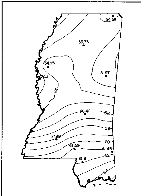
Figure 13. Average annual precipitation pattern in Mississippi.
