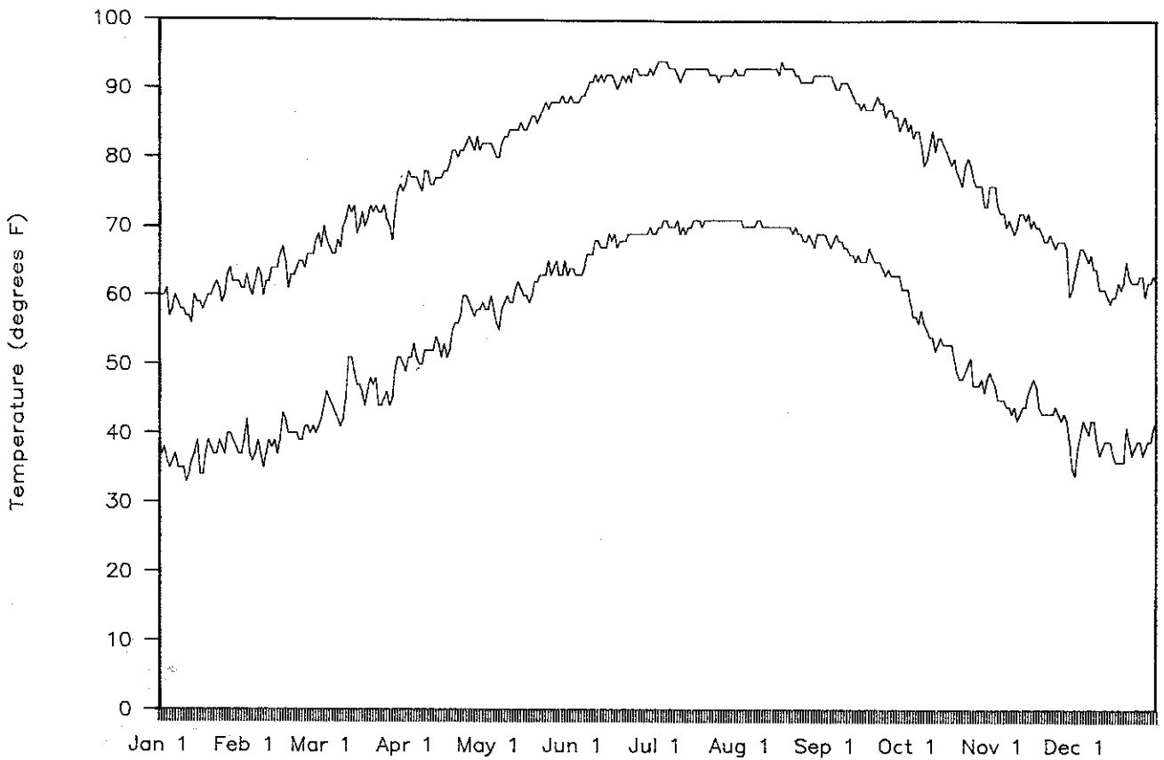
Figure 16. Average daily high and low temperatures, South Mississippi (Hattiesburg).
