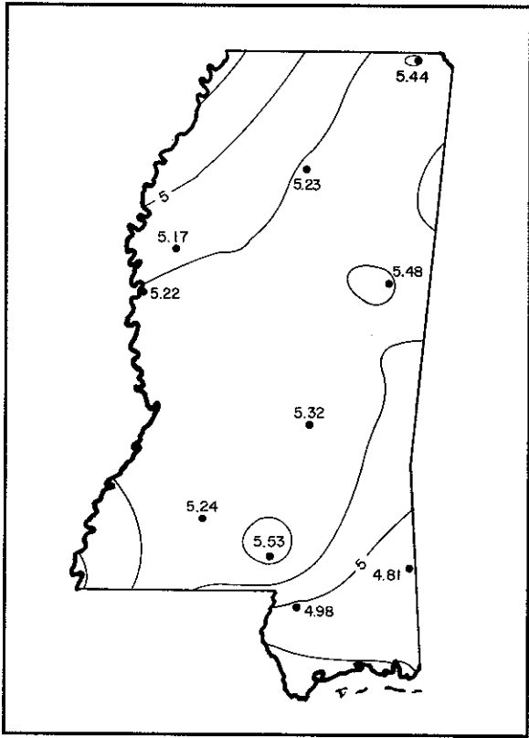
Figure 1. Average monthly precipitation pattern in Mississippi, January.
