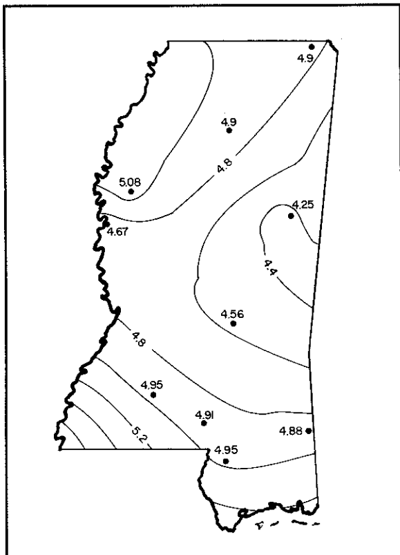
Figure 5. Average monthly precipitation pattern in Mississippi, May.
