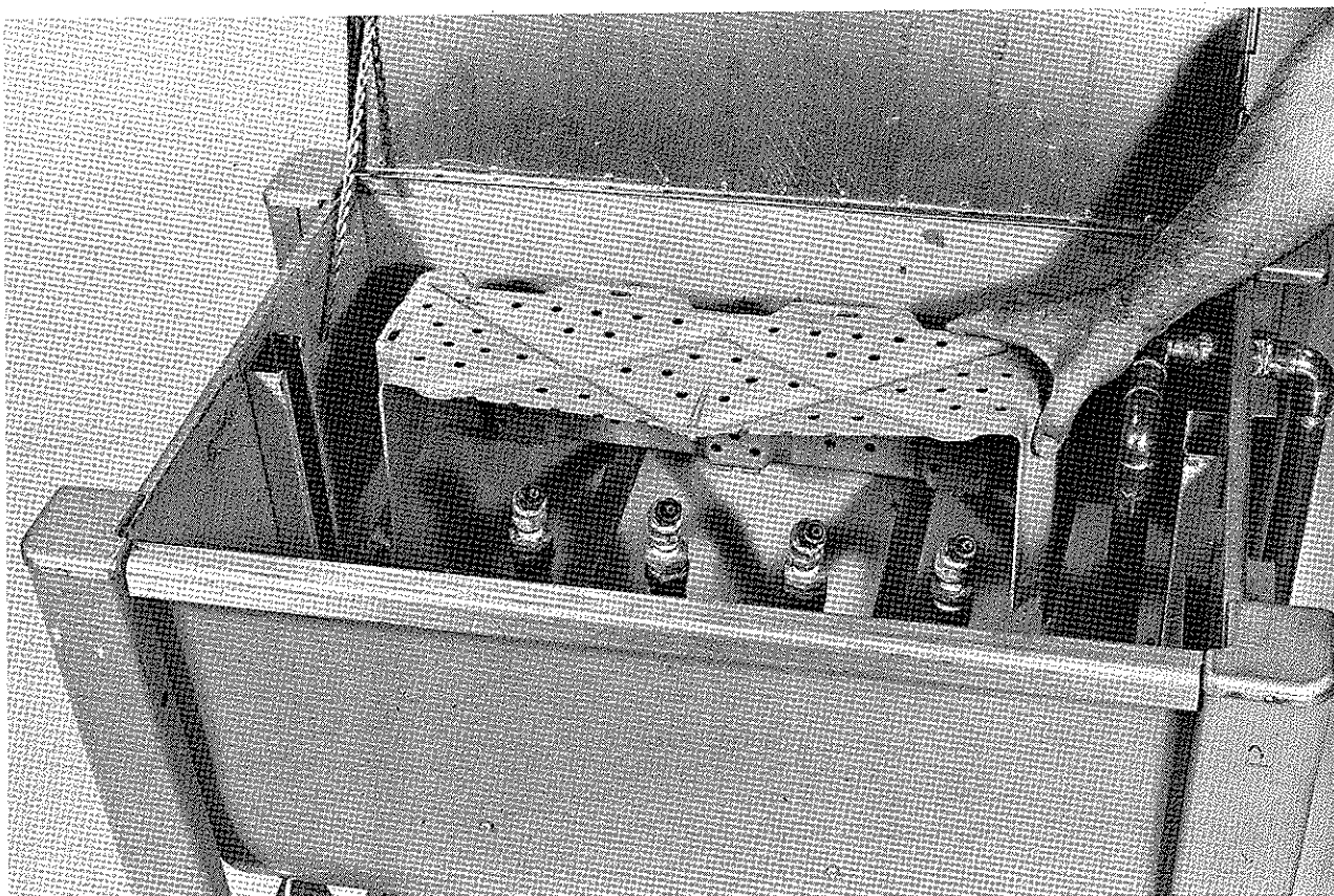
Figure 4. Relationship between nozzles and harvesting container (cutaway).
